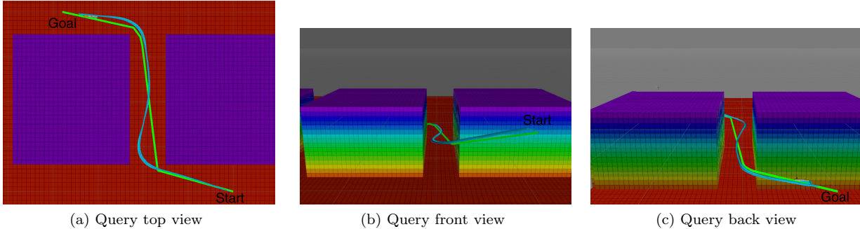
Figure 6: Virtual breakwater structure composed of two obstacles that create a narrow passage, where a start-to-goal query is defined as q_{start} = [x_0, y_0, z_0] and q_{goal} = [x_1, y_1, z_1] . The solution path (in green) is calculated only taking into account geometric constraints. A simulated Sparus II AUV attempted to follow the path, however the resulting trajectory (in light blue) differs from the one calculated, thus leading to risky situations when conducting turning maneuvers.
