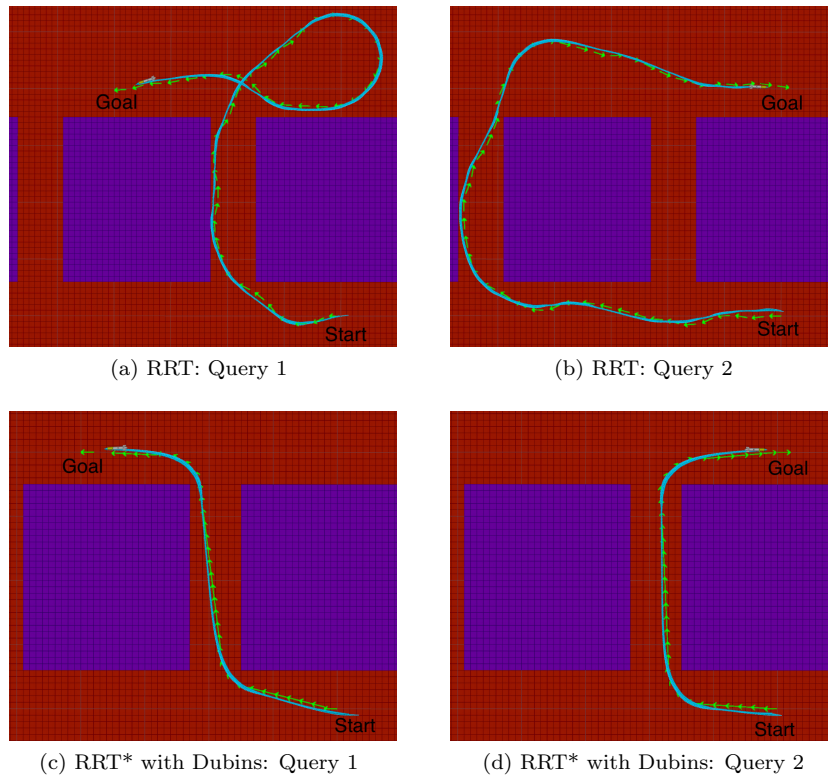
Figure 7: Virtual breakwater structure composed of obstacles that create narrow passages. Sparus II AUV follows the calculated paths. (a), (b) Two different start-to-goal query solutions that were calculated by an RRT algorithm under motion constraints are shown in green. (c), (d) The same start-to-goal queries were solved by an RRT* algorithm with Dubins curves as steering function. Solutions are shown in green.
