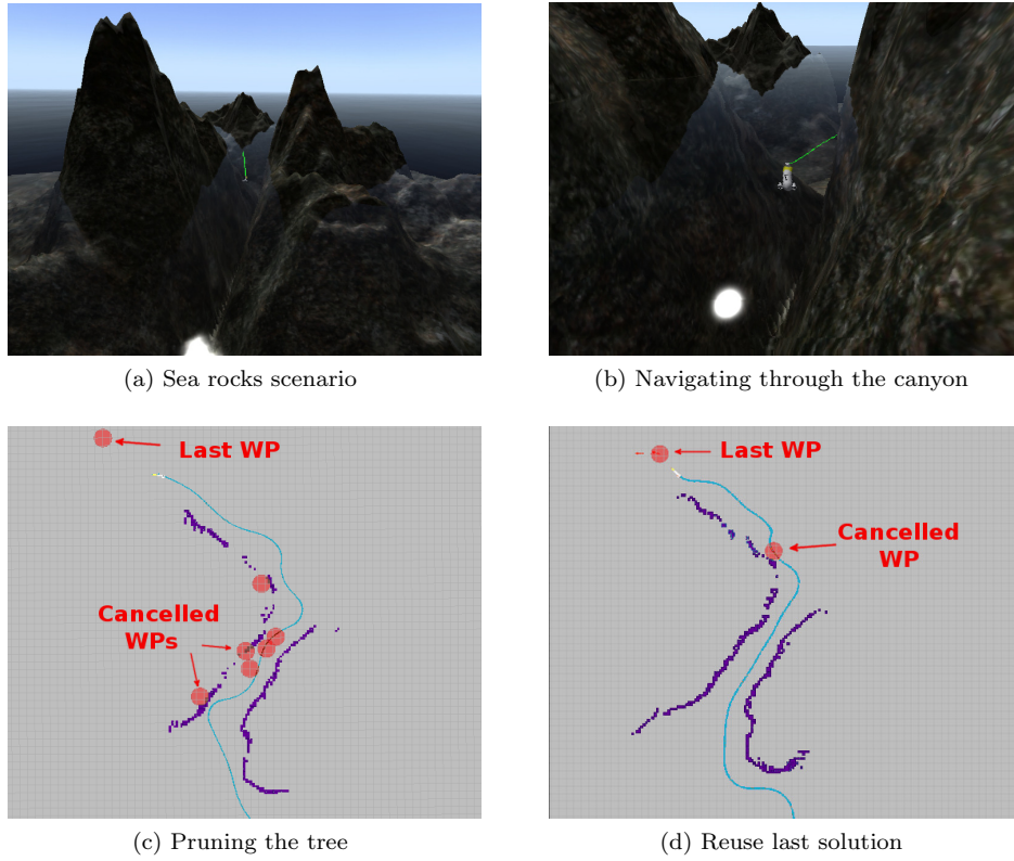
Figure 21: Comparison of the pruning tree scheme and the reuse of the last best known solution when solving start-to-goal queries. The simulated scenario resembles a natural environment. Cancelled waypoints (WPs) are presented as circles in red, and correspond to WPs that may lead the vehicle to a collision, thus requiring the path to be completely replanned.
