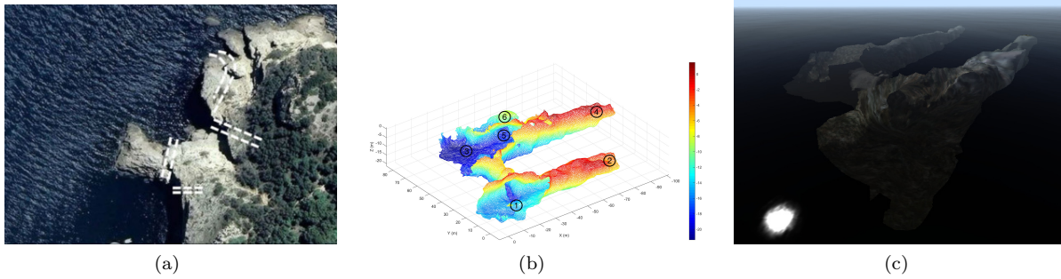
Figure 29: (a) The underwater caves complex “Coves de Cala Viuda” is located in the L’Escal, Spain (Lat: 42.10388, Lon: 3.18255). It consists of three single-branch caves and several tunnels. Their approximate positions are marked with dotted white lines. (b) Meshed map using the SNDC algorithm (Campos et al., 2013). Over the map, the approximate locations of six different goals have been marked in black. Images credit: Mallios et al. 2015 (Mallios et al., 2015; Mallios et al., 2017). (c) Mesh map added into UWSim as a simulation environment.
