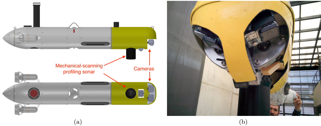
Figure 25: Exteroceptive sensors configuration for the Sparus II AUV to conduct autonomous missions in the underwater canyon. (a) The vehicle was equipped with three GoPro TM Hero 4 Black edition cameras and one mechanical-scanning profiling sonar. (b) Real-world vehicle’s payload.
