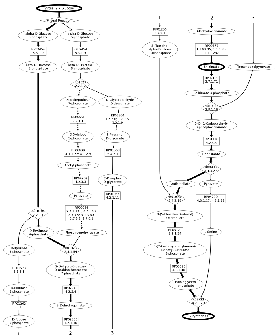
Fig. 4. A single branched pathway result for tryptophan demonstrates how branching schemes can become quite complicated. The bold edges indicate the initial seed pathway, the normal solid lines are the branches attached in the first stage of the algorithm and the dotted line is a final branch added after the initial branches were attached. Compound nodes are ovals, mapping nodes are boxes and reactions are diamonds. The numbers are to assist the reader in following the pathway, as the figure is split in half to fit on the page.
